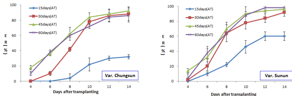
Fig. 3. The emergence rate (ER) of ginseng seedling by GA 3 and alternating temperature (AT) treatments. Vertical bars indicate means \pm SD. GA 3 ; ginseng seedlings were soaked for half an hour at 100 ppm. Var.; variety.
