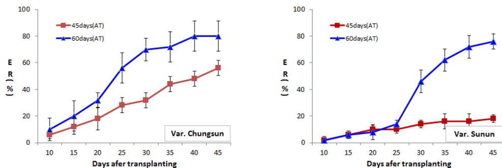
Fig. 2. The emergence rate (ER) of ginseng seedling by no GA 3 and alternating temperature (AT) treatments. Vertical bars indicate means \pm SD. Var.; variety.
